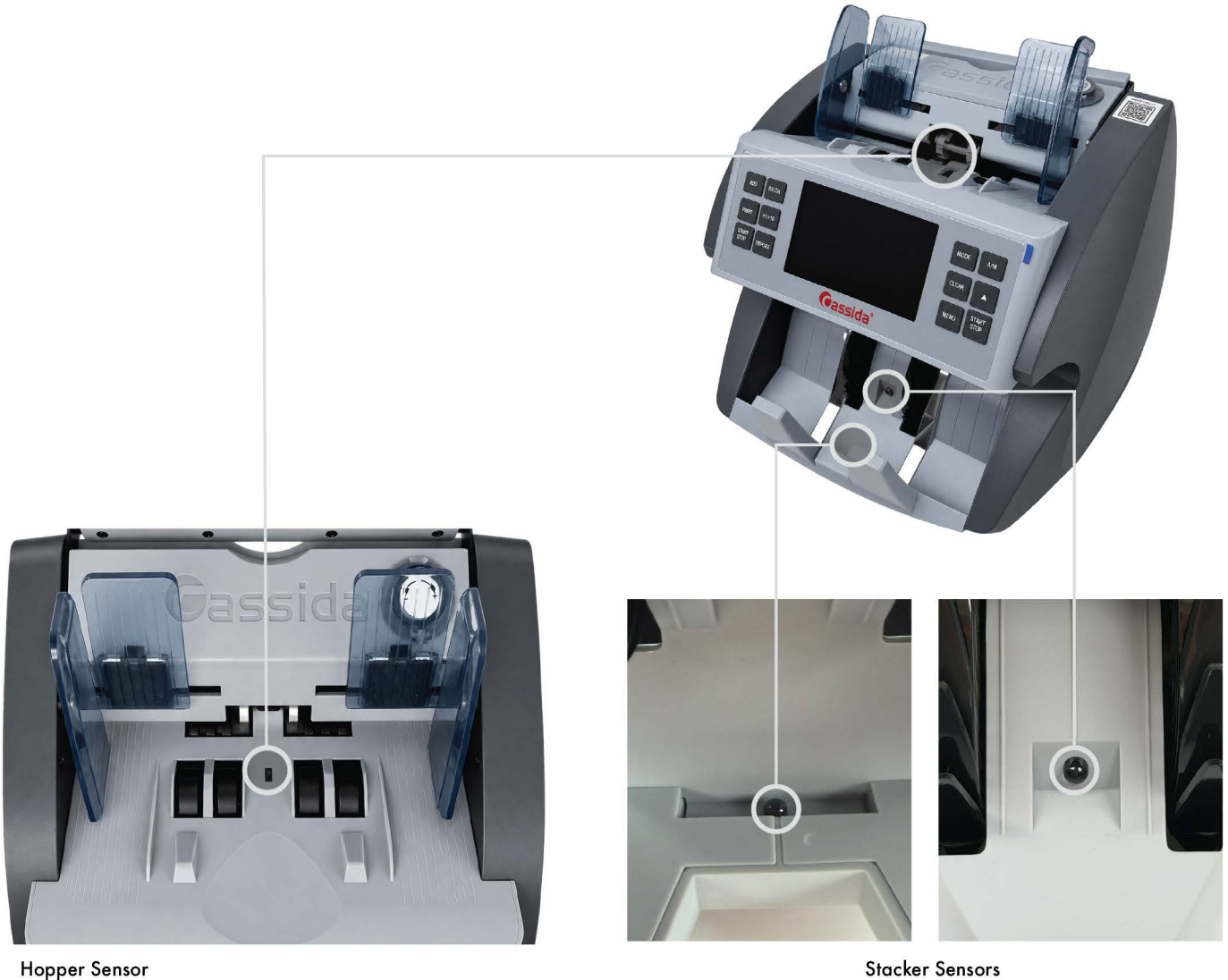
Hopper Sensor
