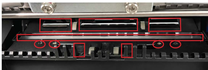
Lower Sensors.
